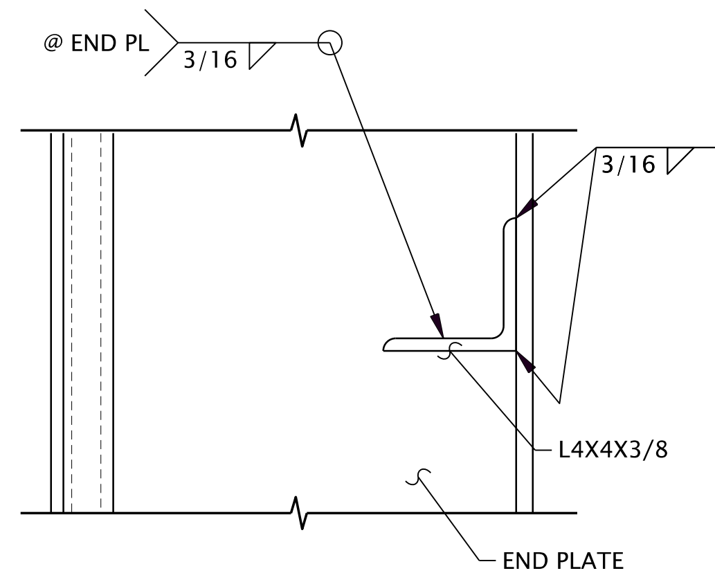
C SECTION S-401 SCALE 3" = 1'-0"
